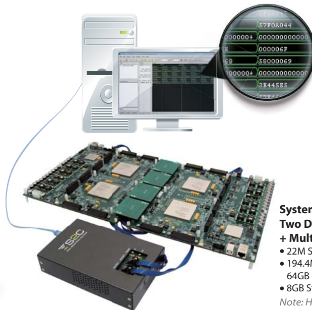
Prodigy™ Multi-Debug Module 2.0 for Xilinx hardware setup
